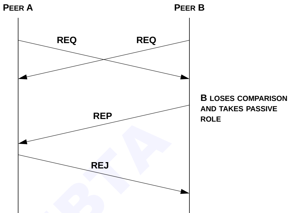
Figure 143 Active/Active, Active Reject
