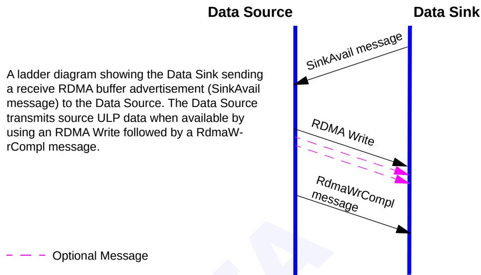
Figure 274 Ladder Diagram for Write Zcopy Mechanism
