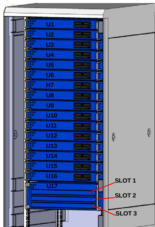
Figure 336 Equipment Rack
