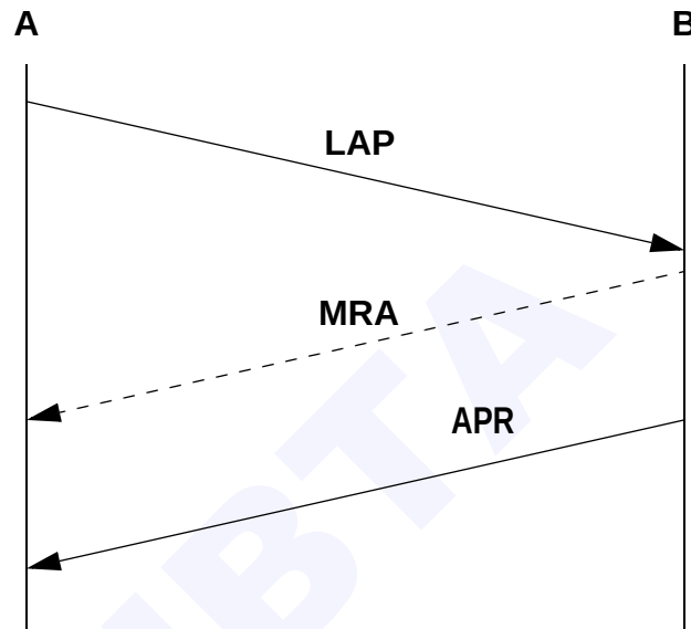
Figure 133 Loading alternate path
