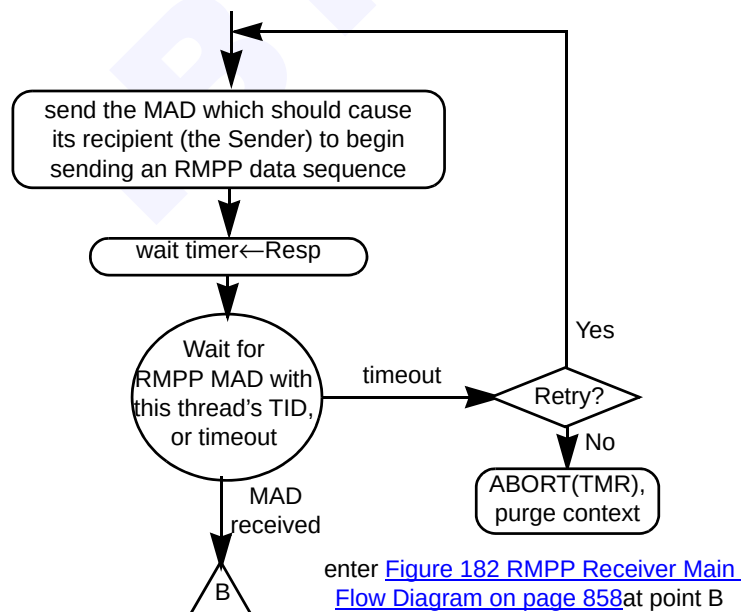
Figure 186 RMPP Receiver-Initiated Flow
