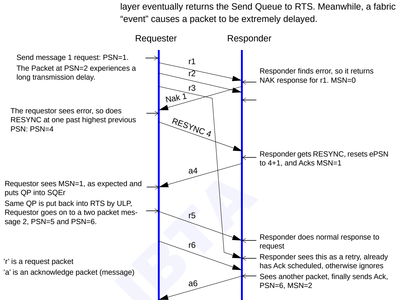
Figure 112 RESYNC prevents corruption by delayed packets
