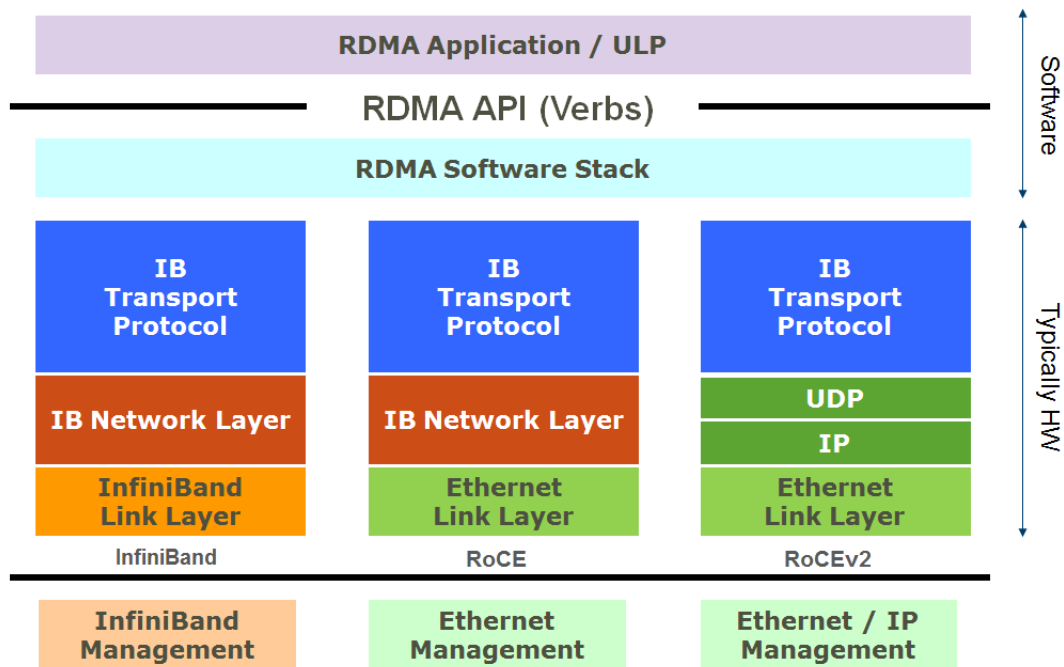
Figure 347 RoCEv2 Protocol Stack
