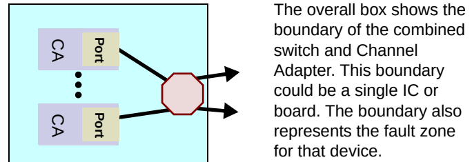
Figure 231 Multiple Single Ported CAs with an Embedded Switch
