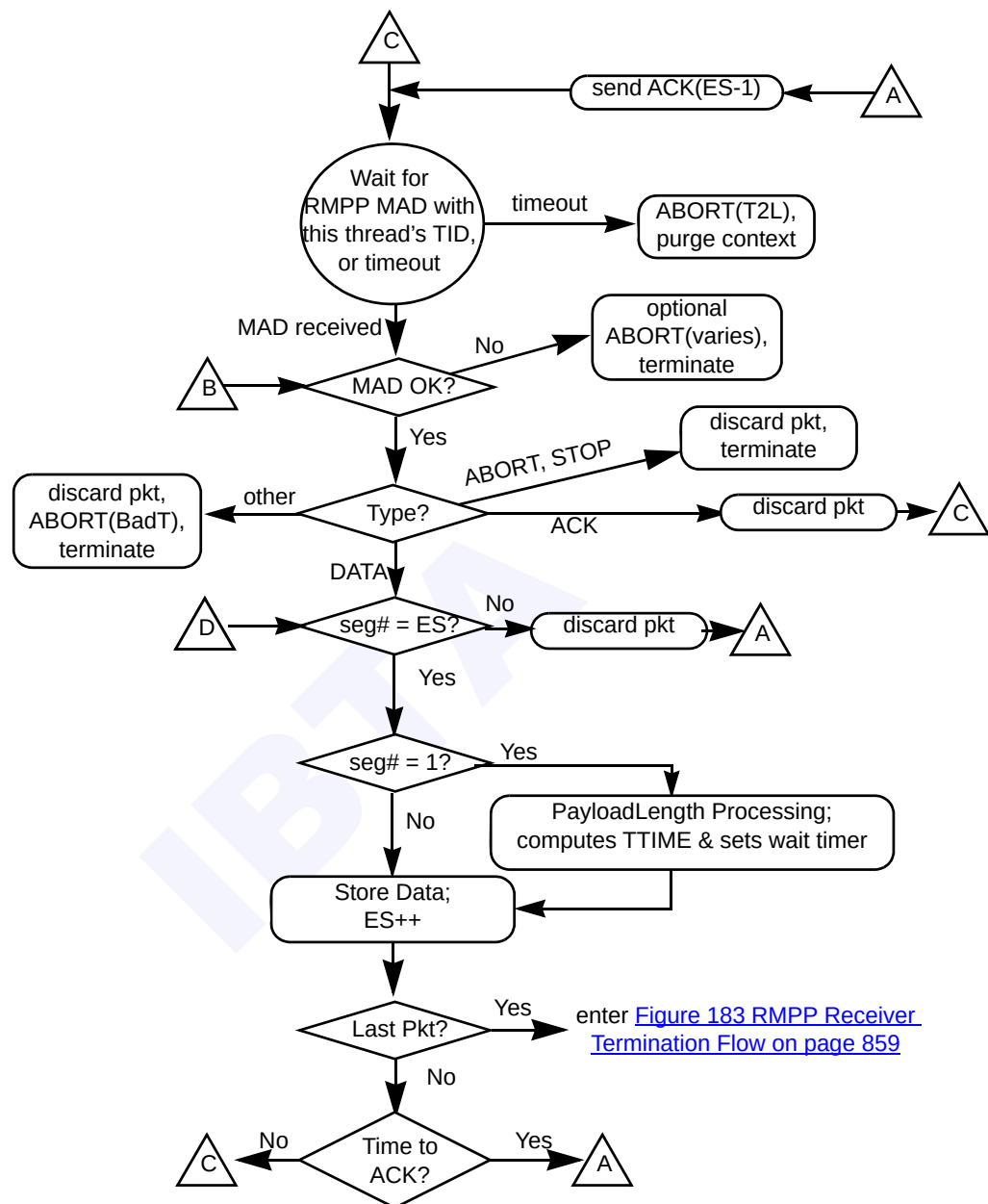
Figure 182 RMPP Receiver Main Flow Diagram
