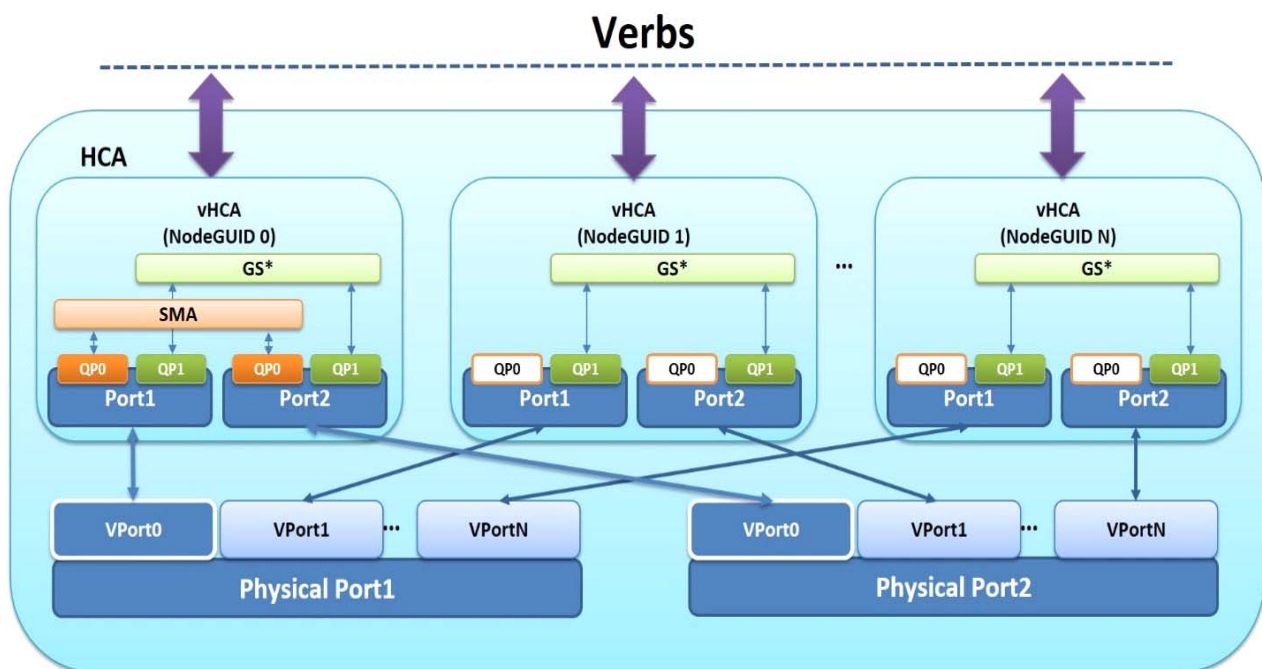
FIGURE 10 Example Virtualized Host Elements
