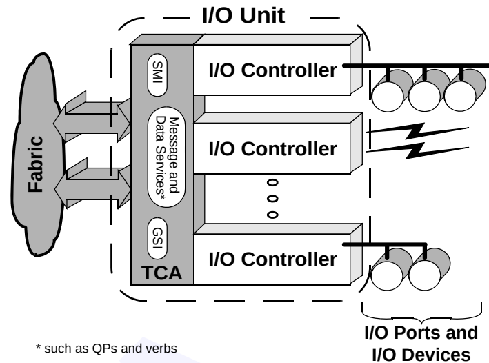
Figure 318 Model for an I/O Unit
