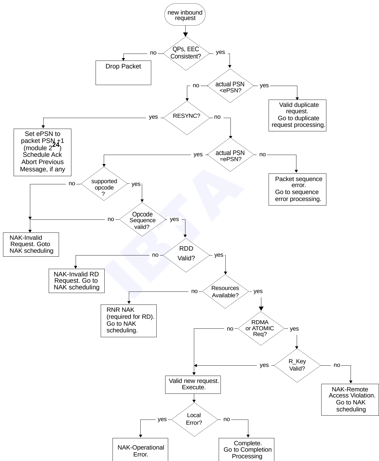
Figure 91 Inbound Request Packet Validation,
