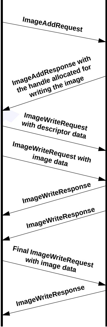
Ladder Diagram of Image Write operation
