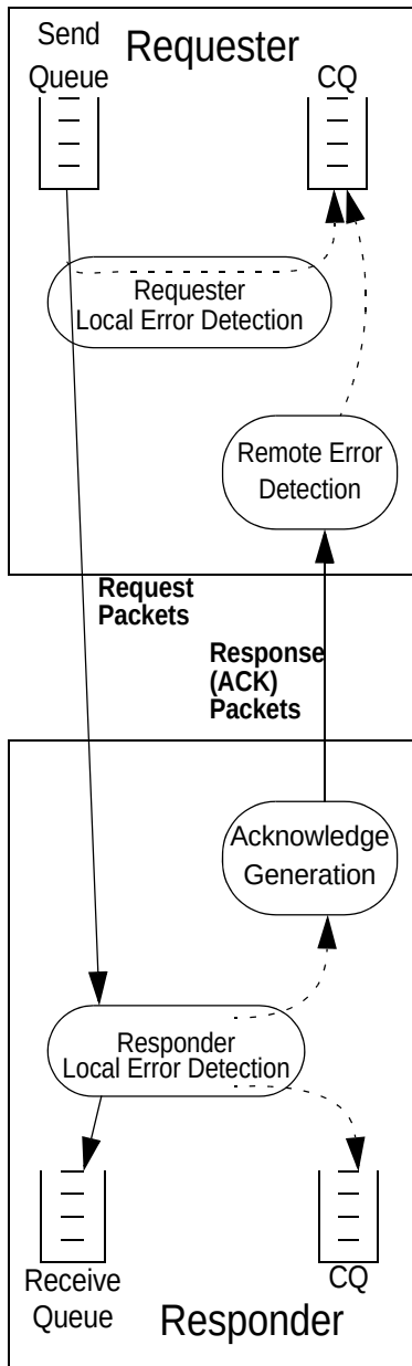
Figure 118 Requester/Responder Error Detection
