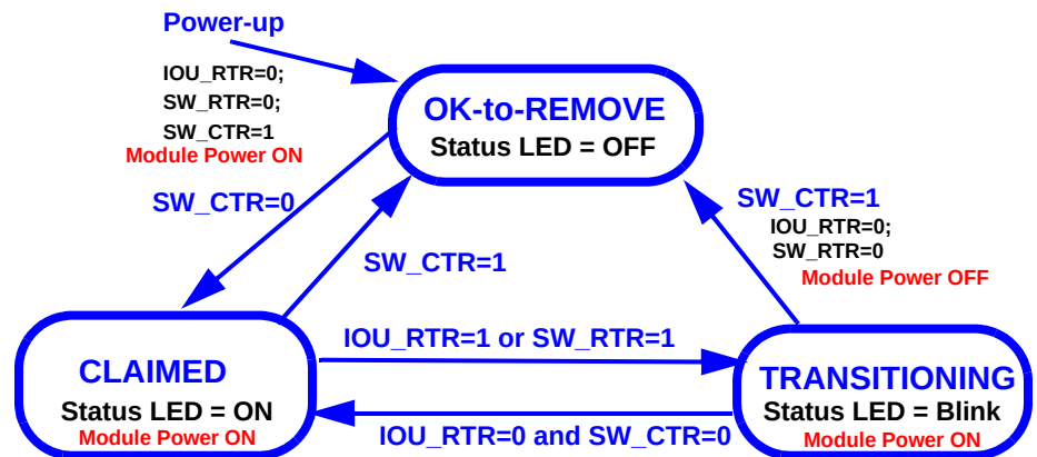
Figure 331 Graceful Removal State Diagram
