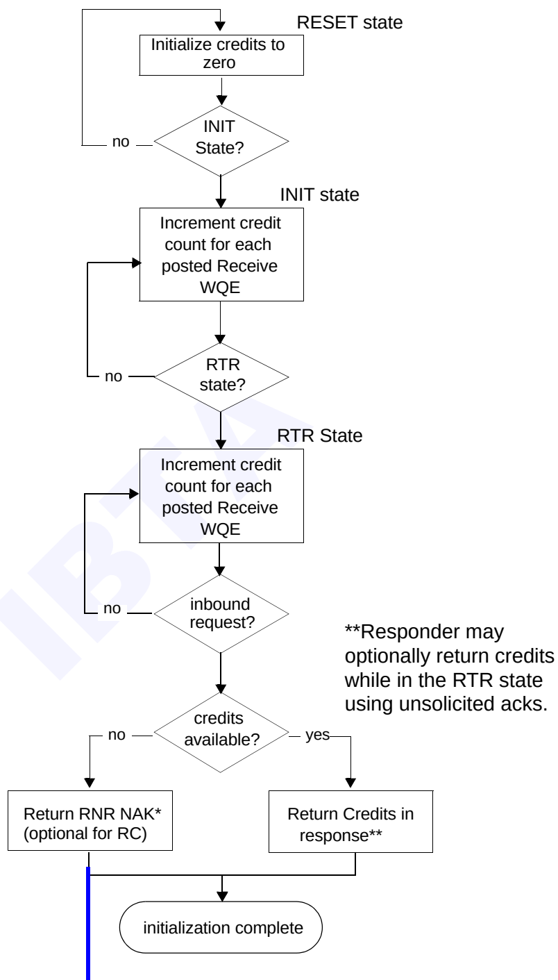
Figure 106 Responder End-to-End Credit Initialization
