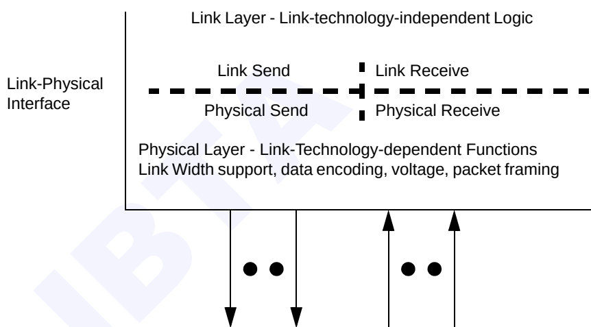
Figure 49 Physical Functions and Physical/Link Interface
