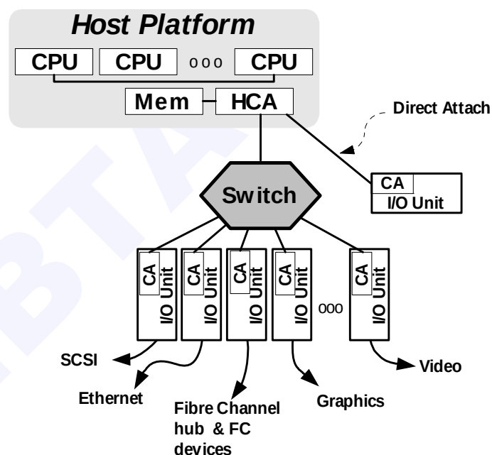
Figure 237 Single System & Direct Attached I/O
