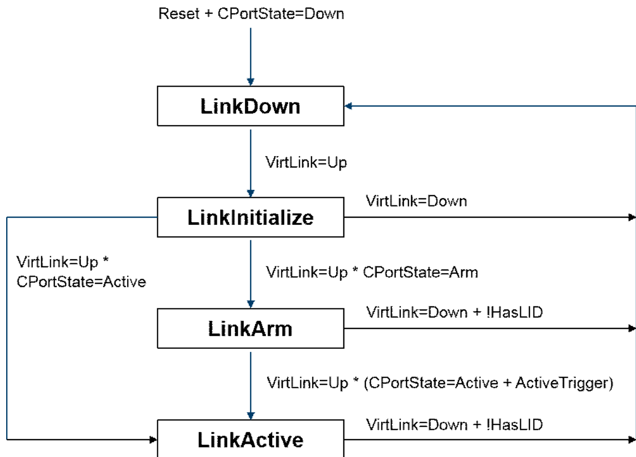
FIGURE 11 VPort PortState state machine
