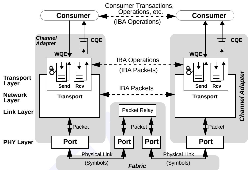
Figure 13 IBA Communication Stack
