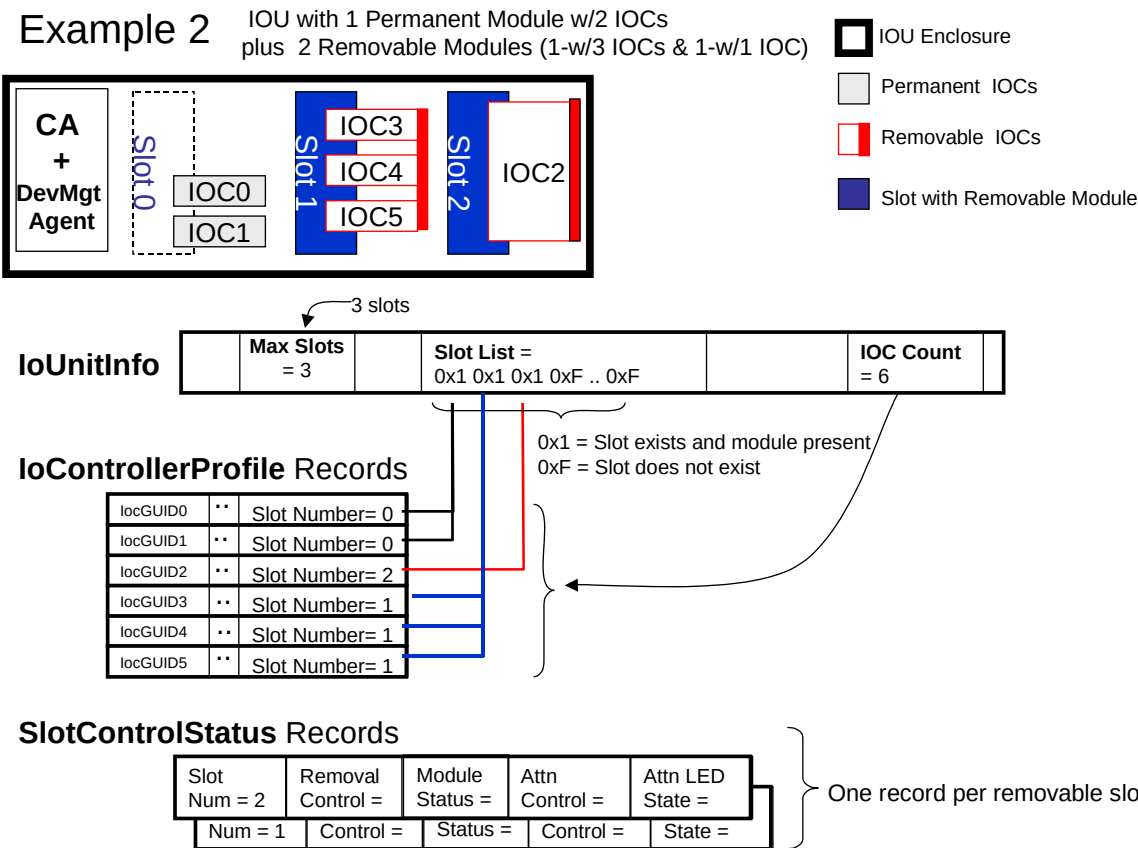
Figure 324 Example of IOU with Removable Modules
