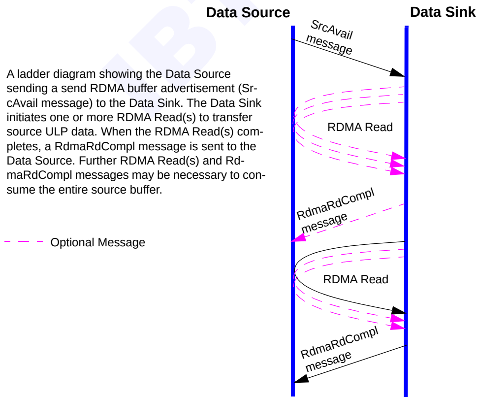
Figure 273 Ladder Diagram for Read Zcopy Mechanism
