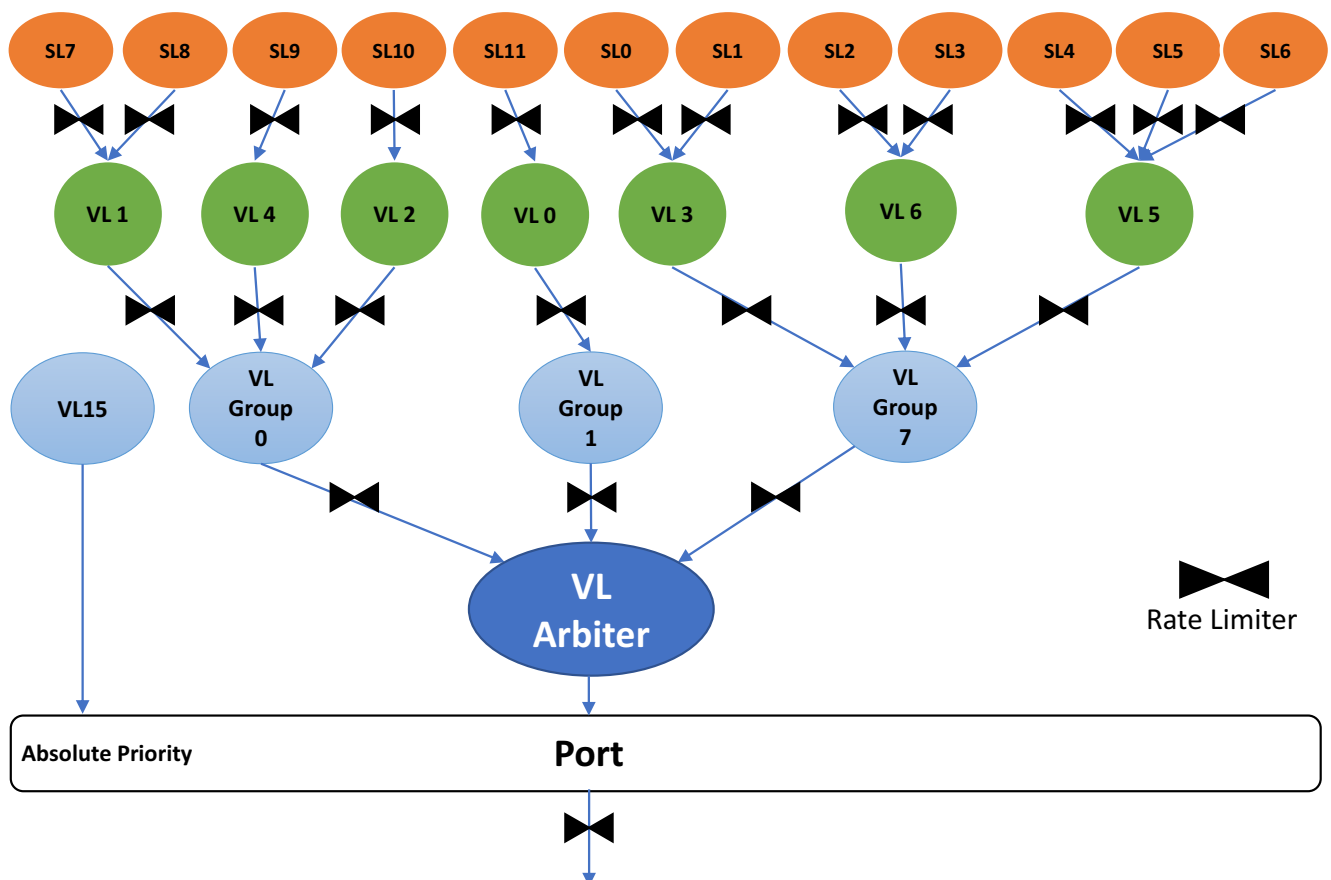
Figure 54 SL to Port Level Arbitration Scheme
