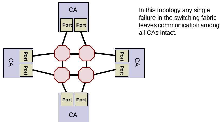
Figure 229 Fault Tolerant Connection to a Single
