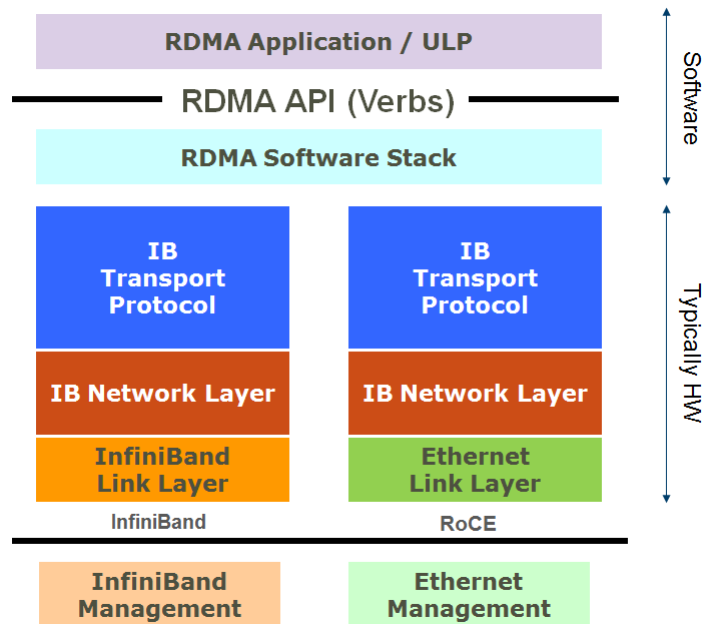
Figure 344 InfiniBand and RoCE Protocol Stacks
