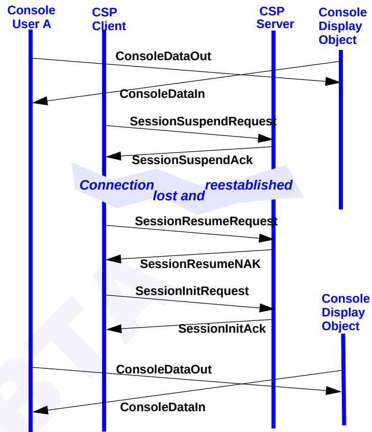
Figure 247 Resume Reject
