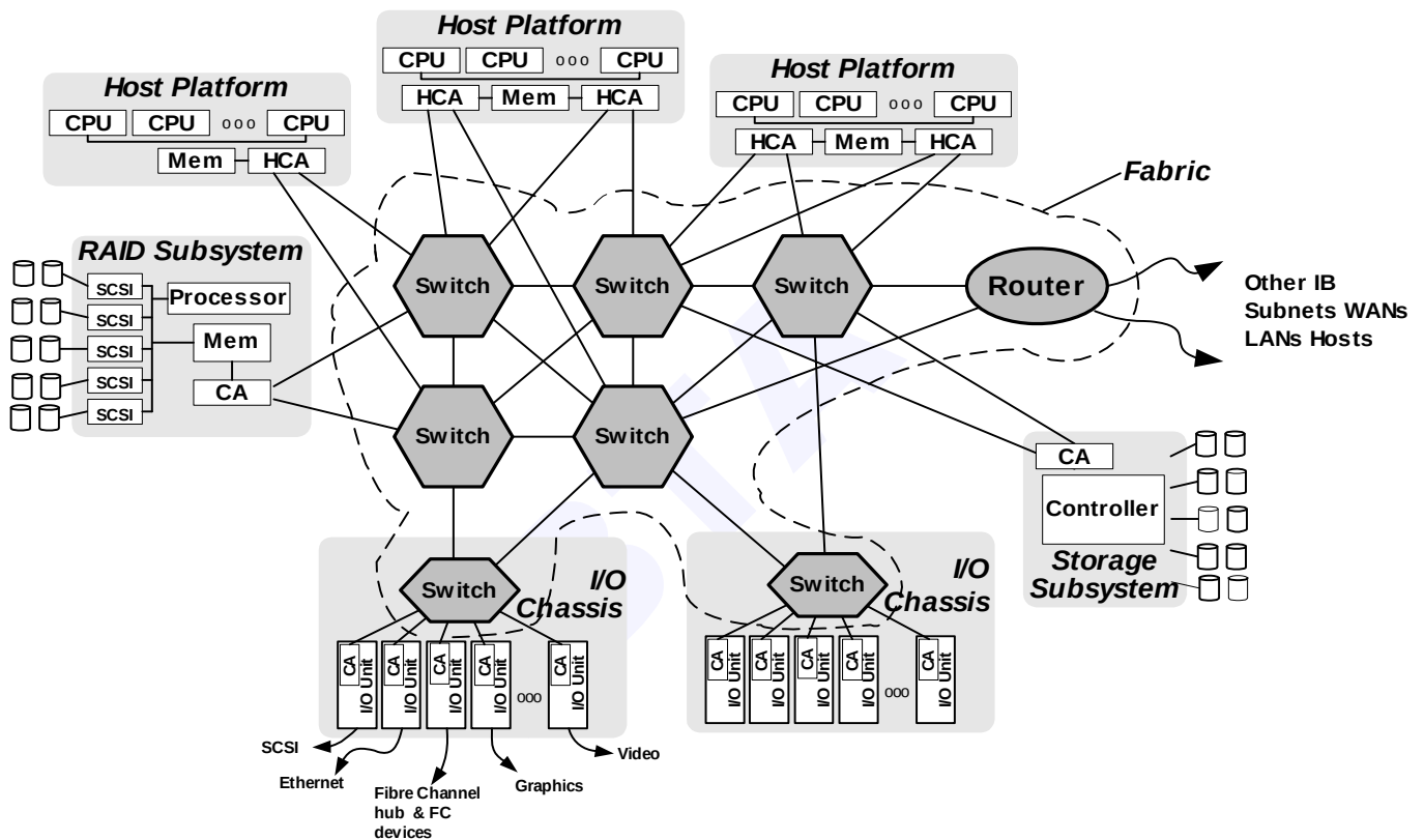
Figure 238 Multiple Systems
