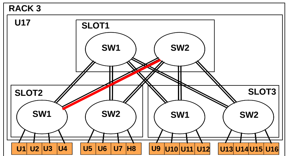
Figure 338 Physical hierarchy view
