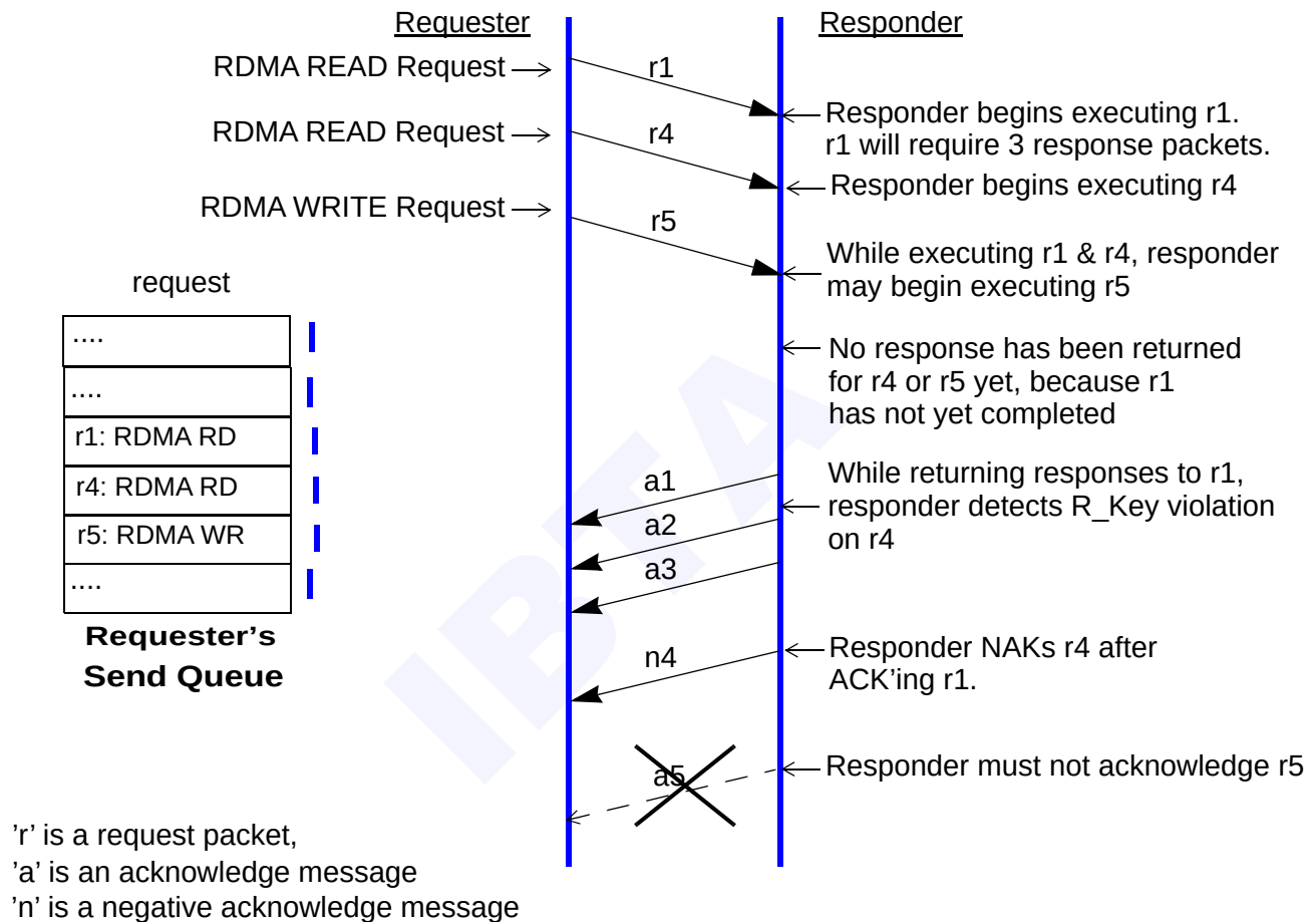
Figure 94 Relaxed Ordering Rules for RDMA READS
