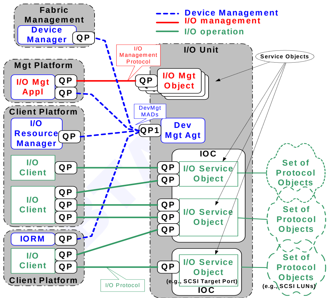
Figure 319 I/O Components and Relationships
