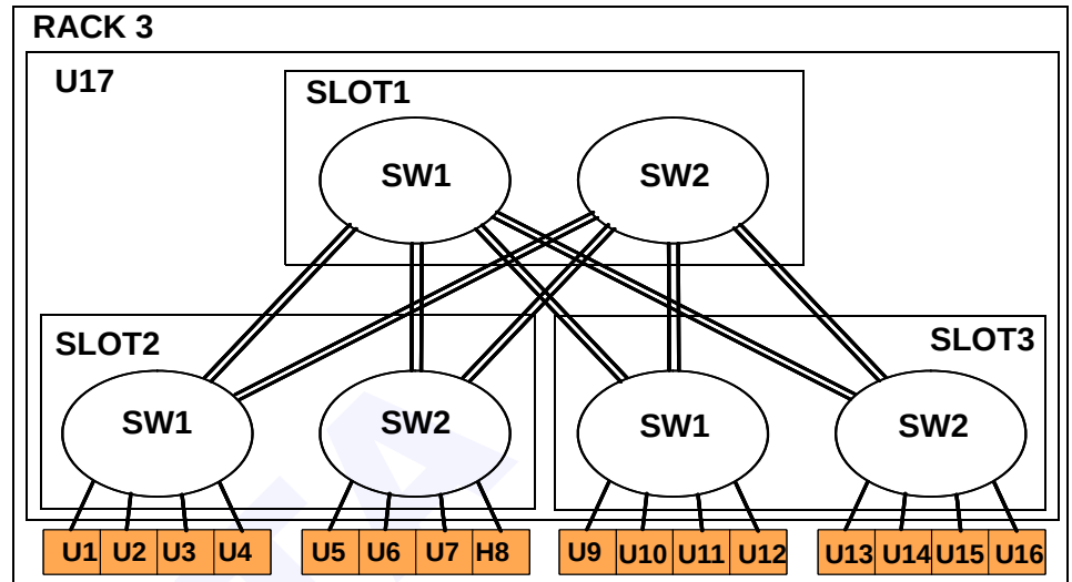
Figure 341 Physical hierarchy view
