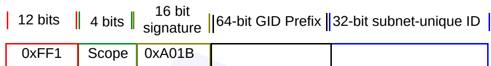
Figure 203 SA-Created Multicast GID
