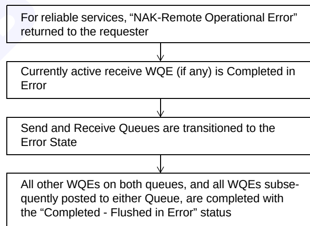
Figure 122 Transport Class A Responder Behavior
