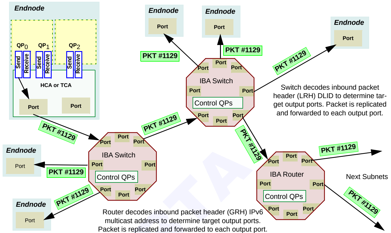
Figure 21 Example Unreliable Multicast
