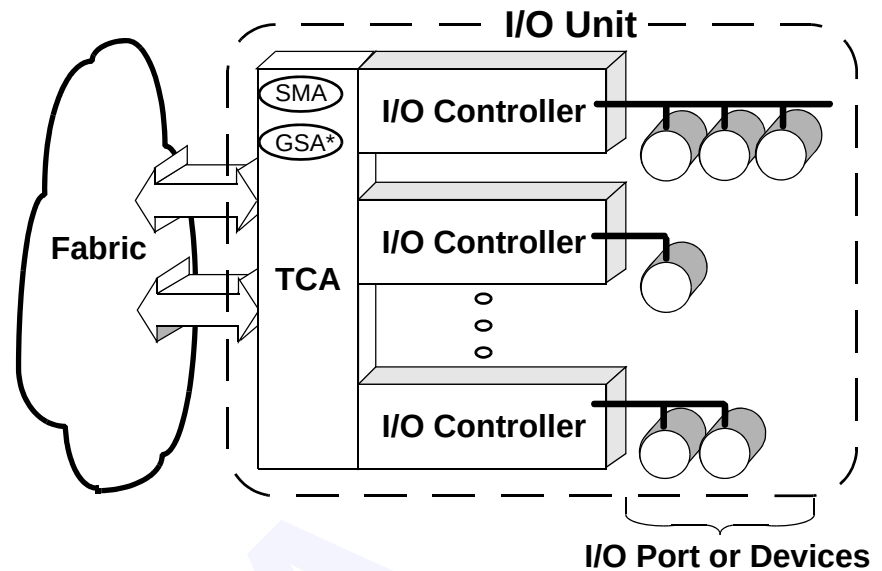
Figure 35 I/O Unit
