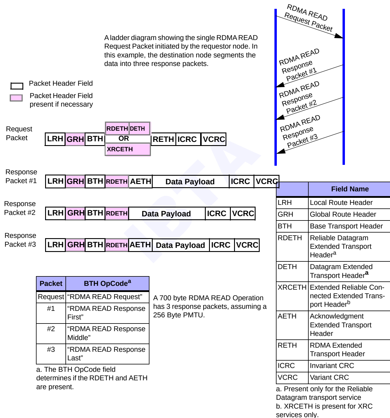
Figure 79 RDMA READ Operation
