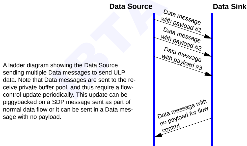
Figure 272 Ladder Diagram for BCopy
