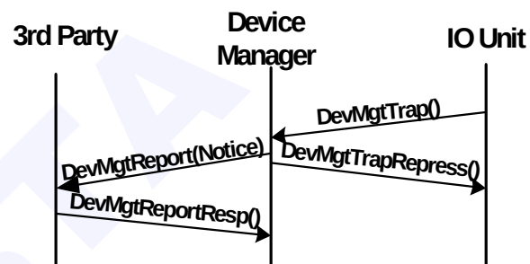
Figure 310 Trap Forwarding
