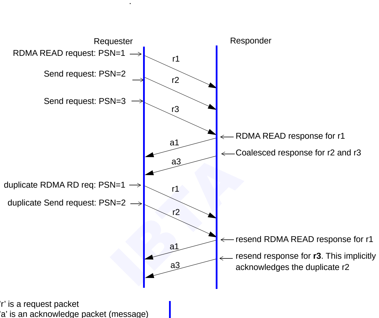
Figure 97 Acknowledging a Duplicate RDMA READ Request
