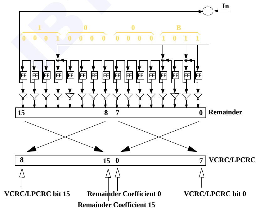
Figure 58 VCRC / LPCRC Generator
