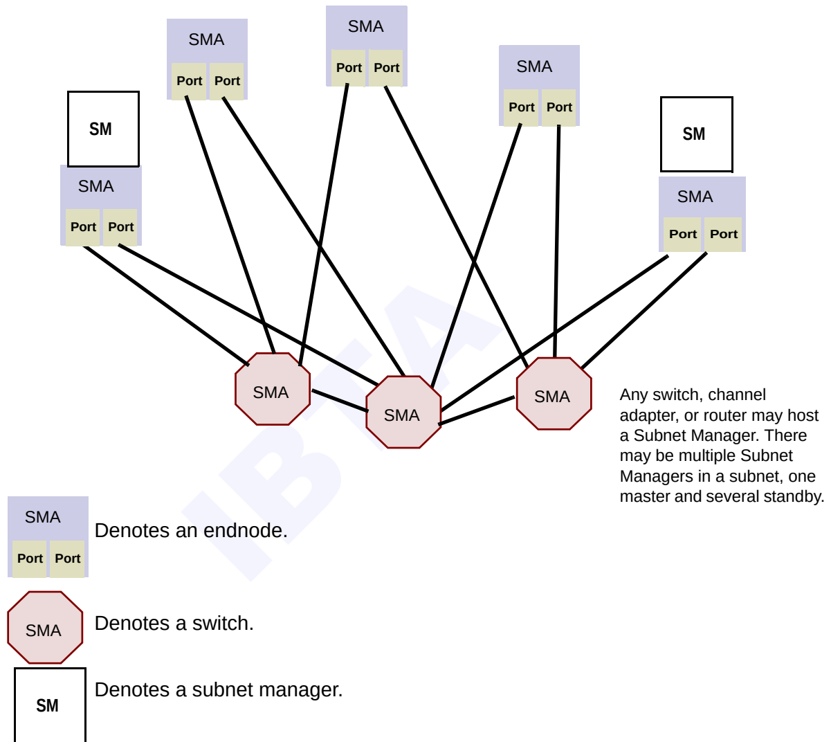
Figure 147 Typical Subnet Manager/Agent
